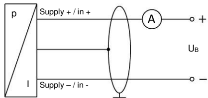
Fig. 4: Connection circuit diagram
