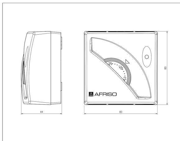
TA 03 without switch, with lamp
