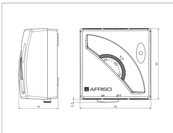
TA 03 with switch, with lamp
