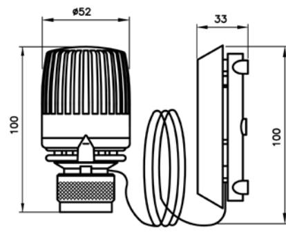
Thermostat control head 323 KD with remote probe, Danfoss clamp connection
